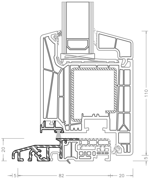
Soglia ALU 82 mm – art. 252555
